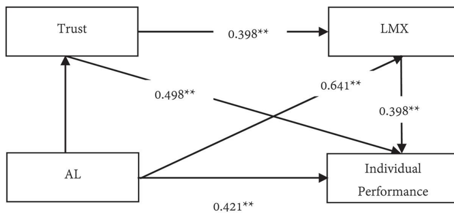
Figure 2. Structural Model
