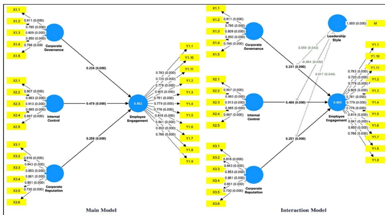
Figure 2. Bootstrapping results
